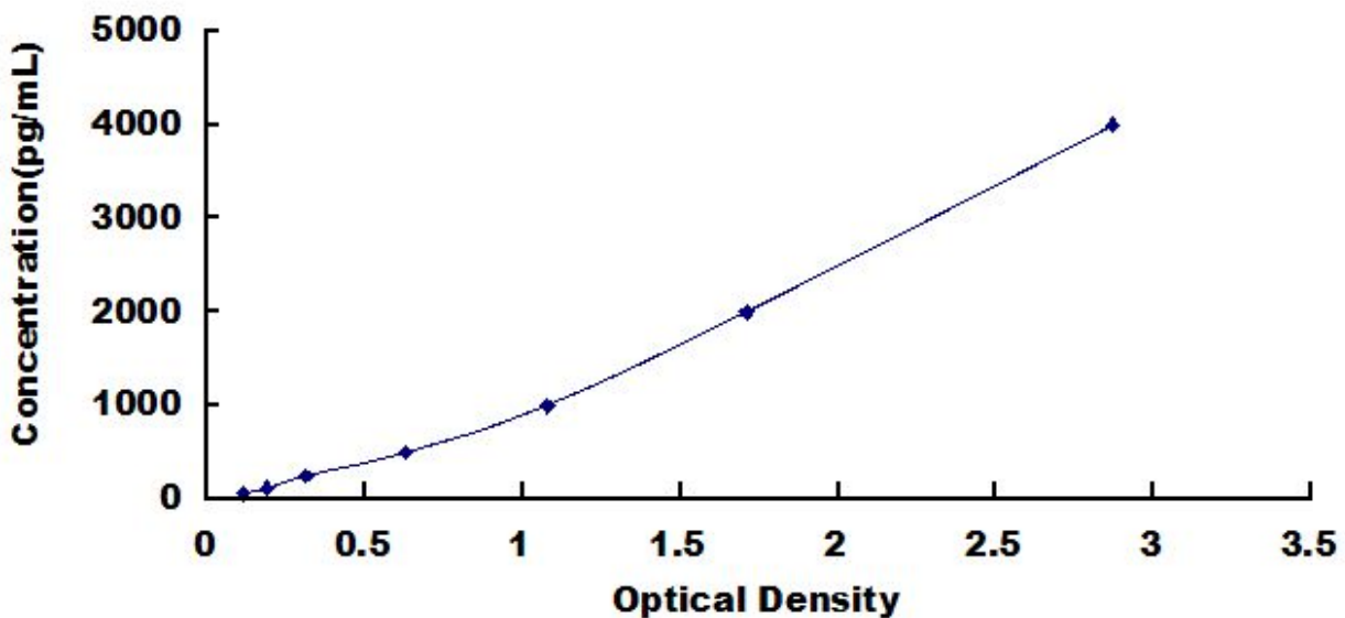
Typical Standard Curve for CRP, Human ELISA.
